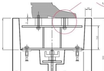
Original plan of plinth
